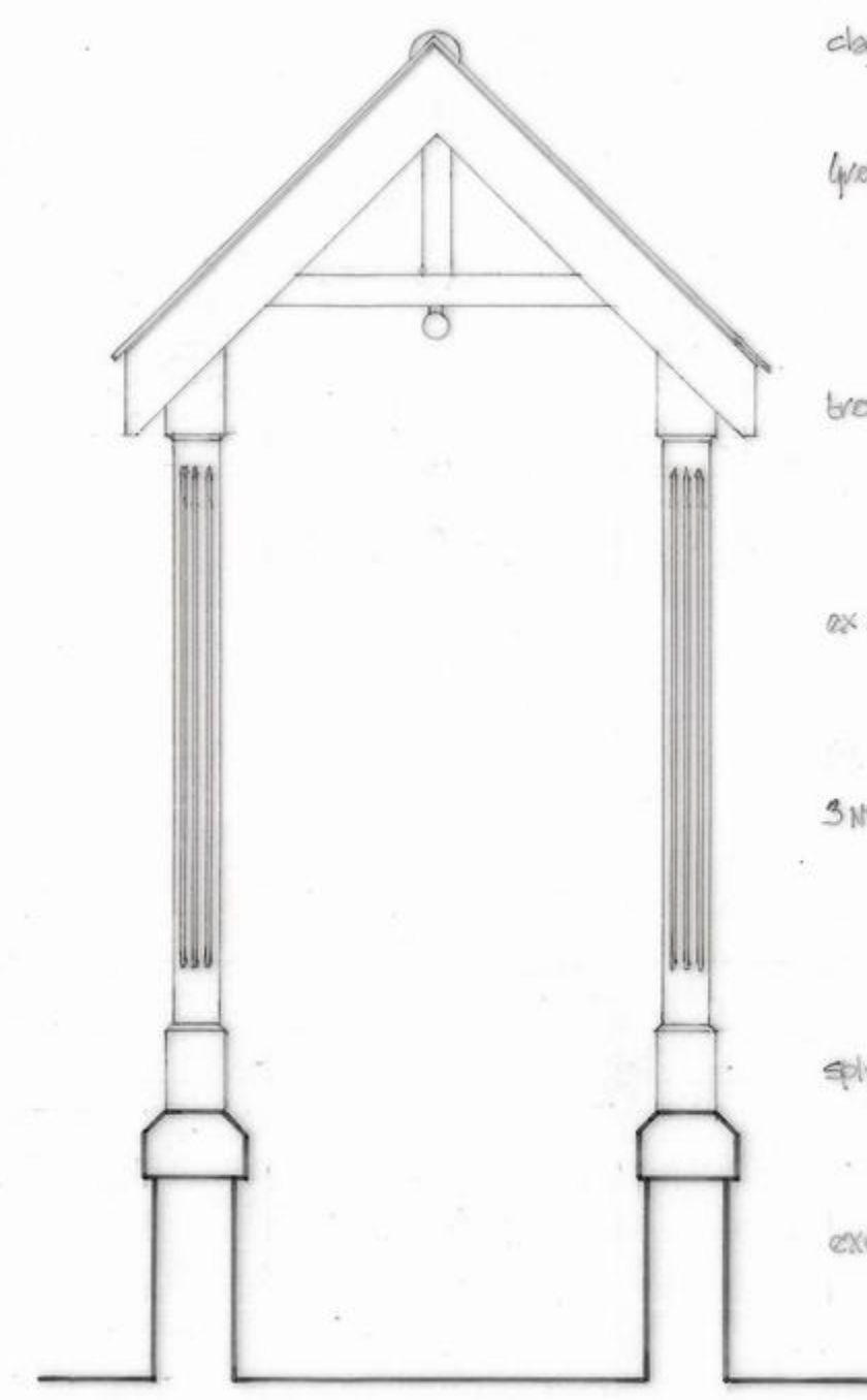
Porch Details. 1:20
