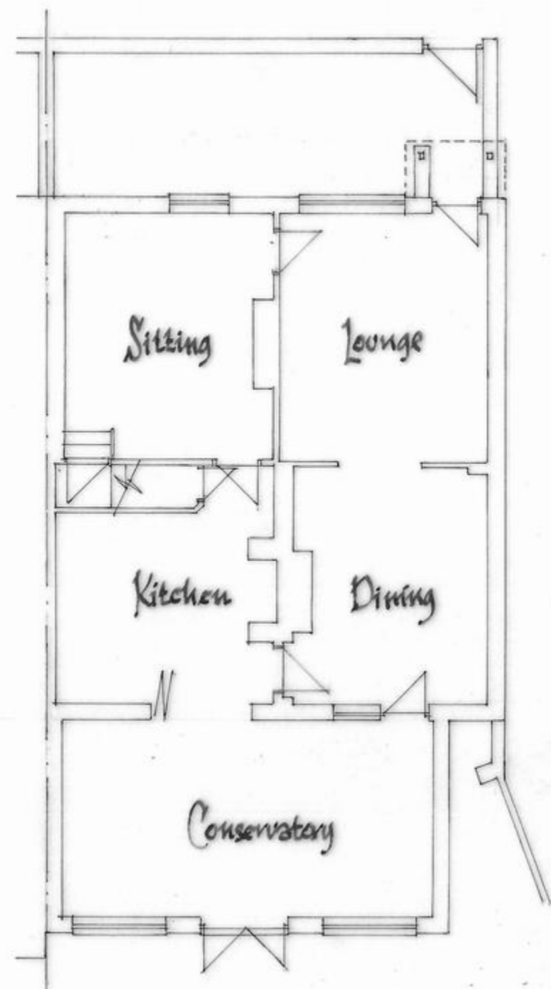
Proposed Plan
